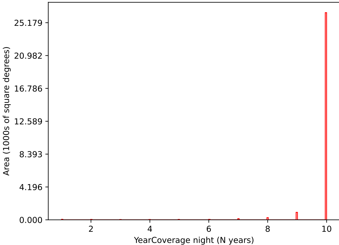
weather_cloudso0v3.4_10yrs i band: YearCoverage night
