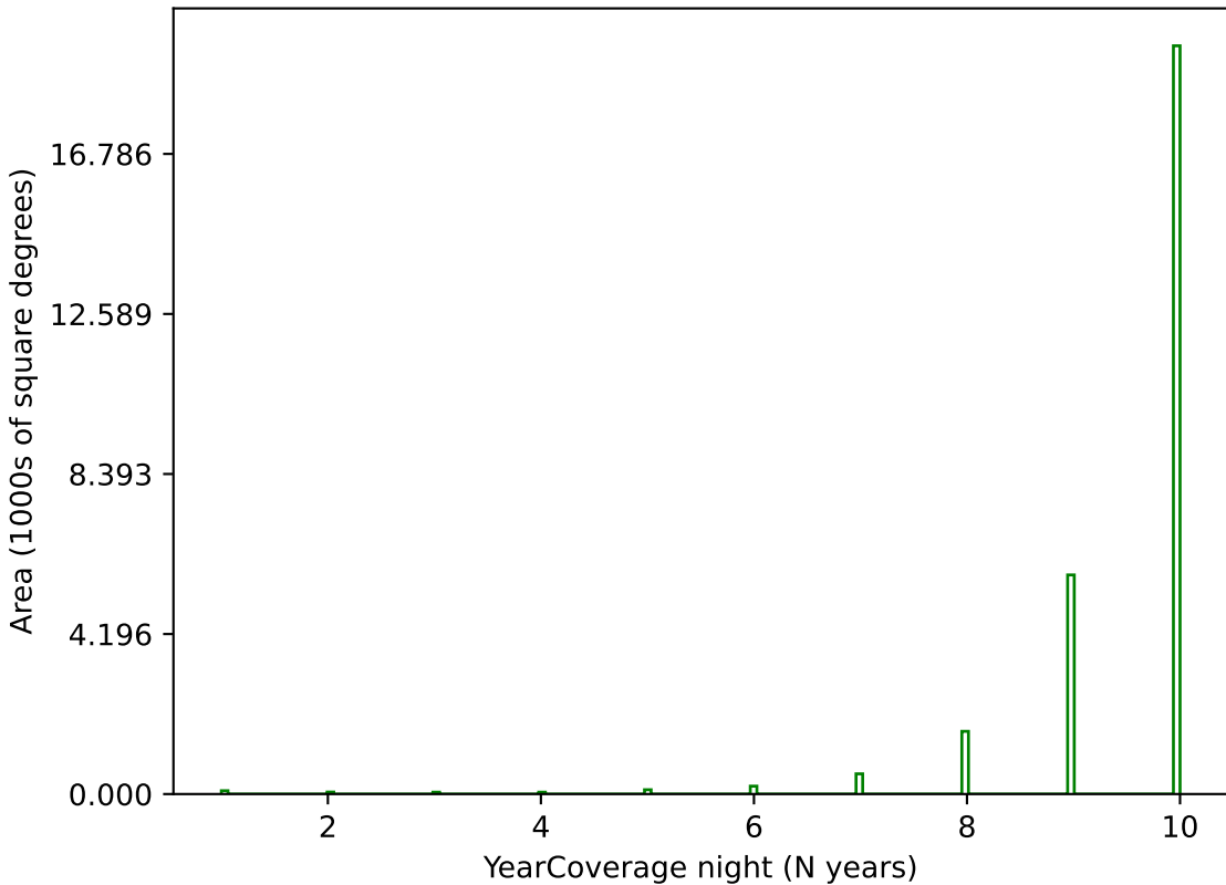
weather_cloudso0v3.4_10yrs g band: YearCoverage night
