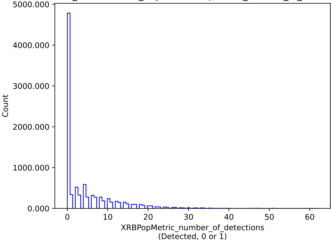
weather_cloudso0v3.4_10yrs : XRBPoMetric_number_of_detections
