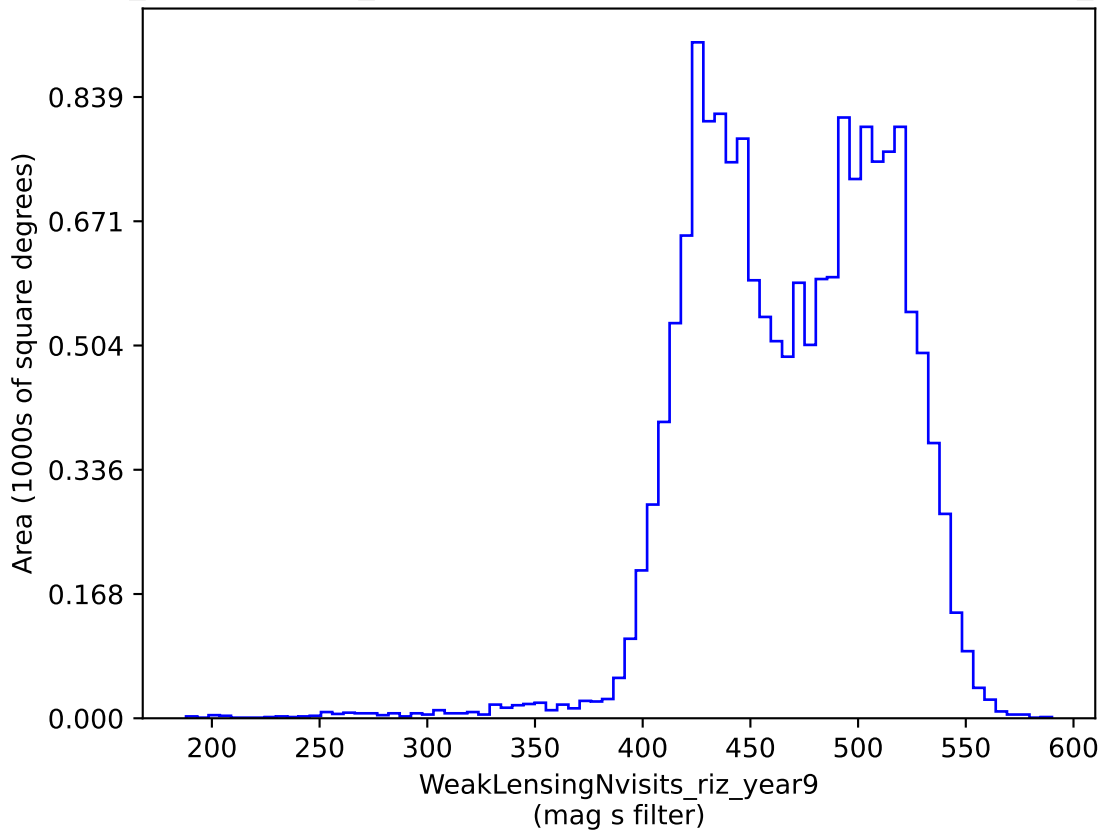
weather_cloudso0v3.4_10yrs gri band non-DD: WeakLensingNvisits_riz_year9
