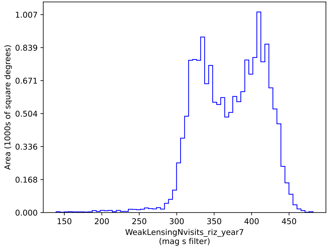
weather_cloudso0v3.4_10yrs gri band non-DD: WeakLensingNvisits_riz_year7
