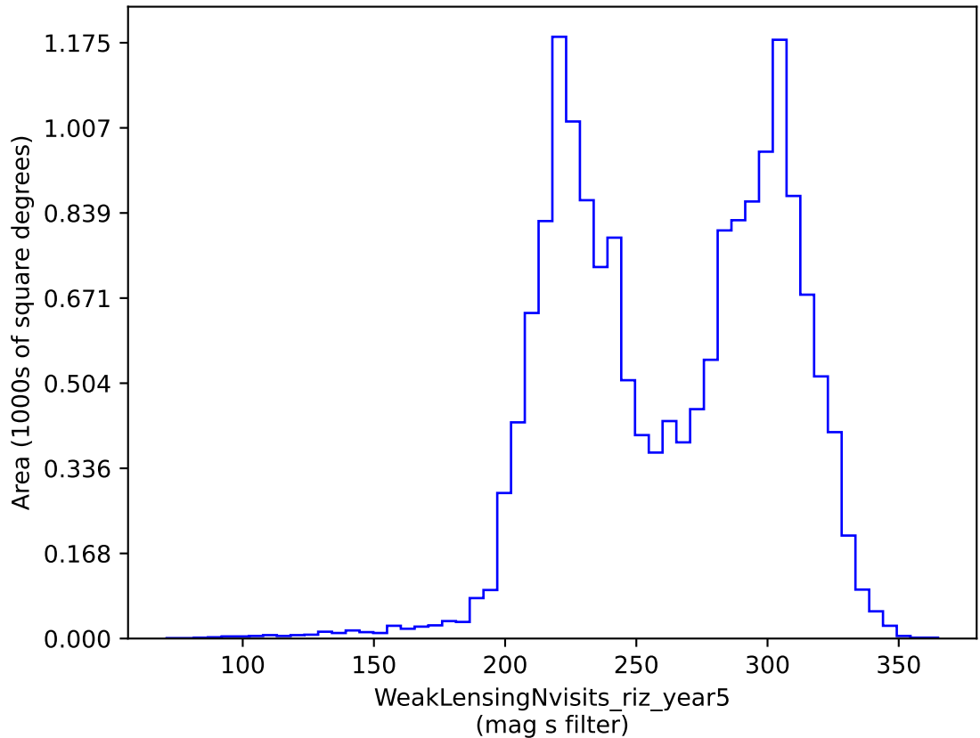
weather_cloudso0v3.4_10yrs gri band non-DD: WeakLensingNvisits_riz_year5
