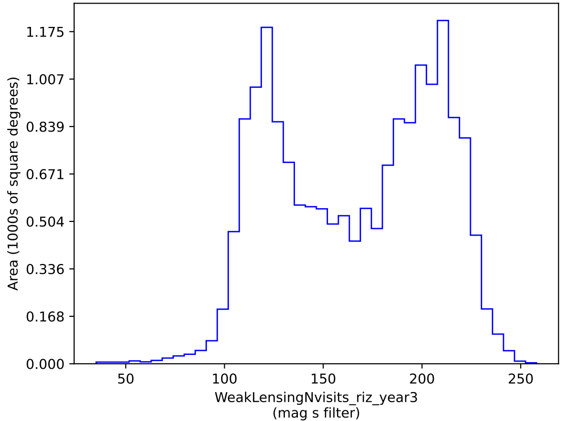
weather_cloudso0v3.4_10yrs gri band non-DD: WeakLensingNvisits_riz_year3
