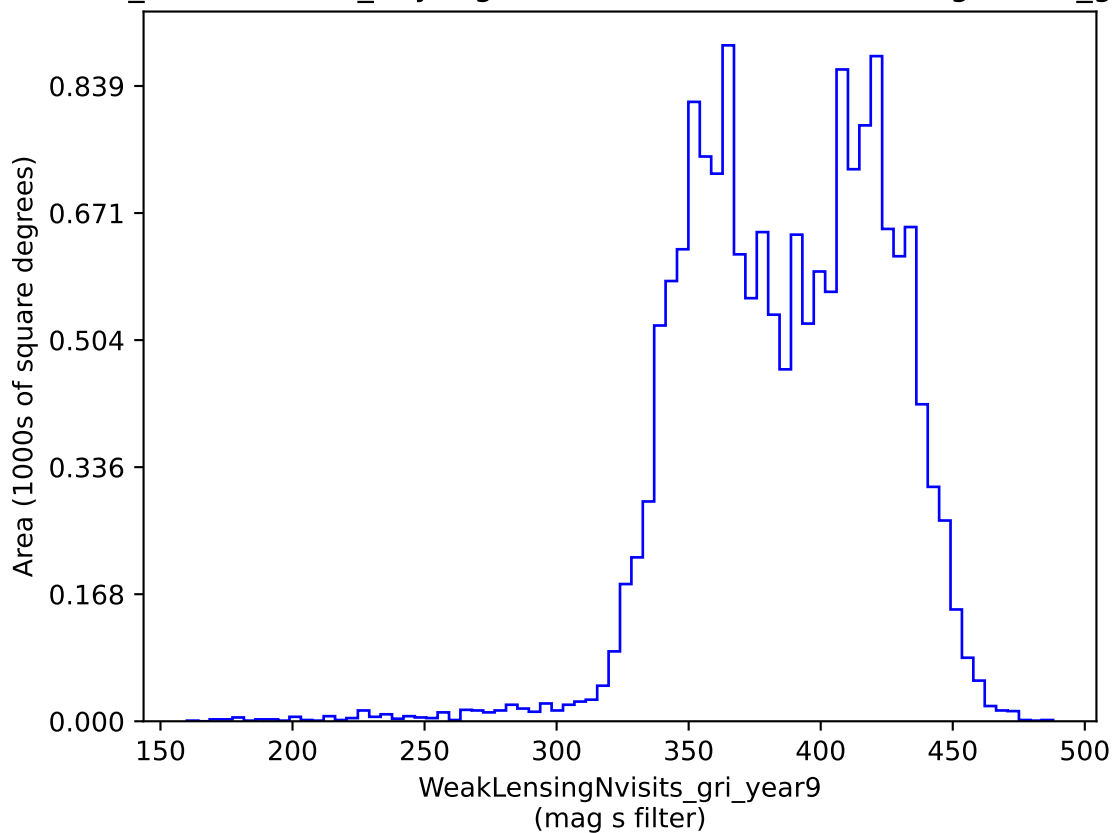
weather_cloudso0v3.4_10yrs gri band non-DD: WeakLensingNvisits_gri_year9
