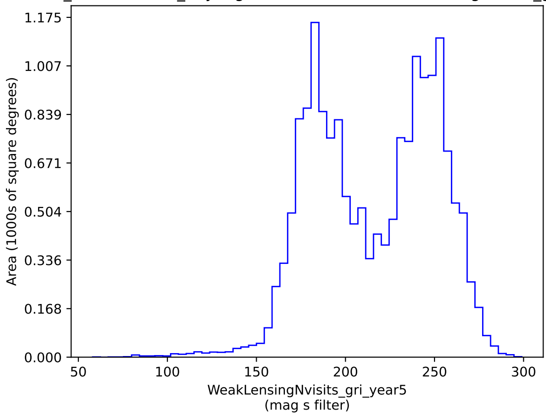
weather_cloudso0v3.4_10yrs gri band non-DD: WeakLensingNvisits_gri_year5
