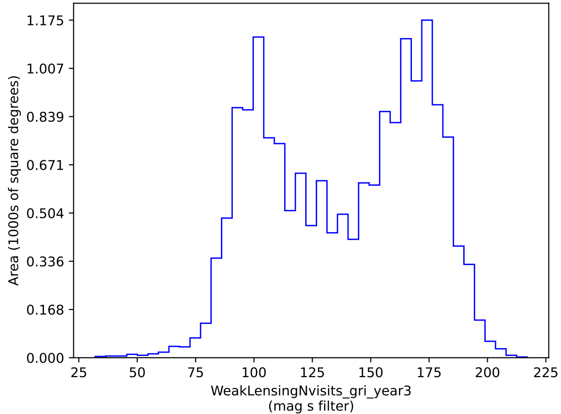
weather_cloudso0v3.4_10yrs gri band non-DD: WeakLensingNvisits_gri_year3
