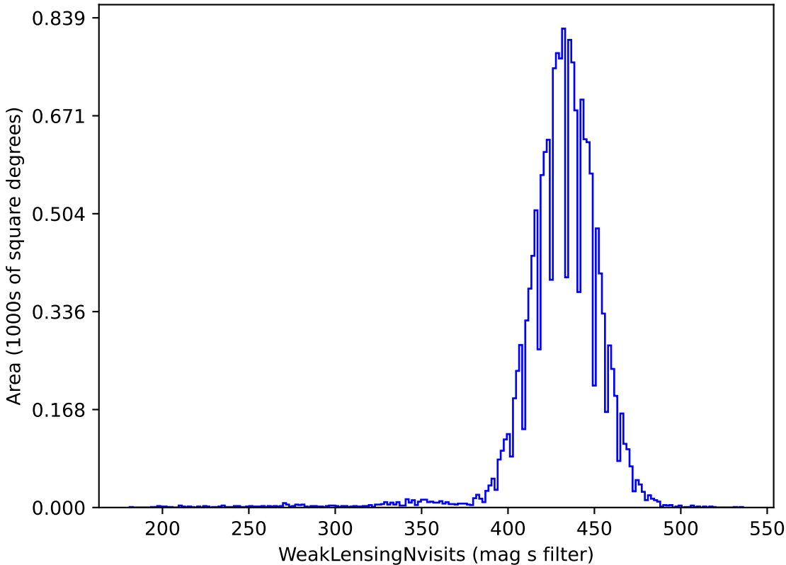
weather_cloudso0v3.4_10yrs gri band non-DD: WeakLensingNvisits
