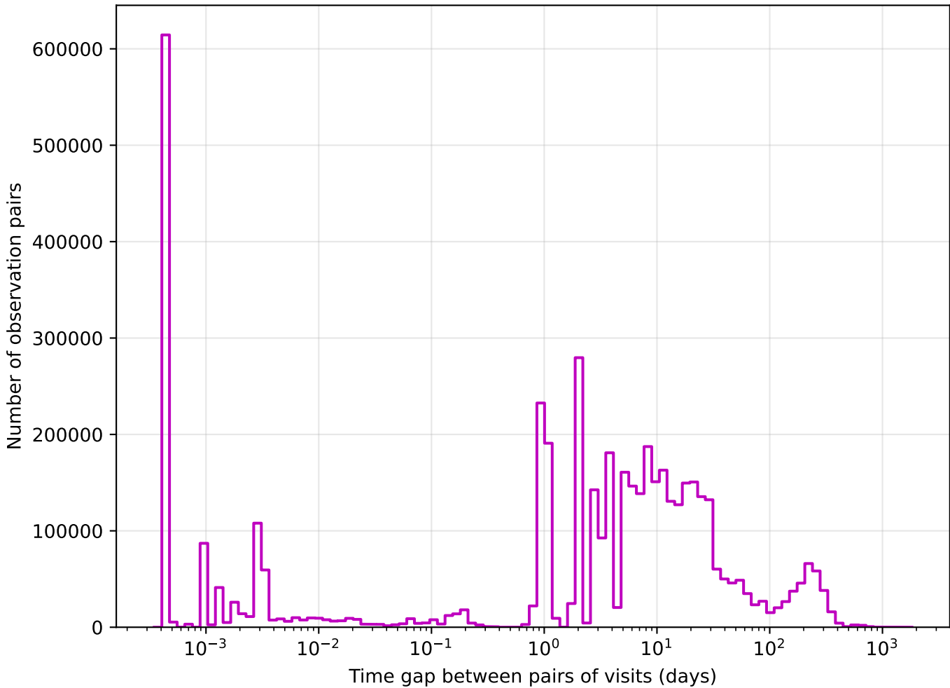
weather_cloudso0v3.4_10yrs z band: Tgaps observationStartMJD
