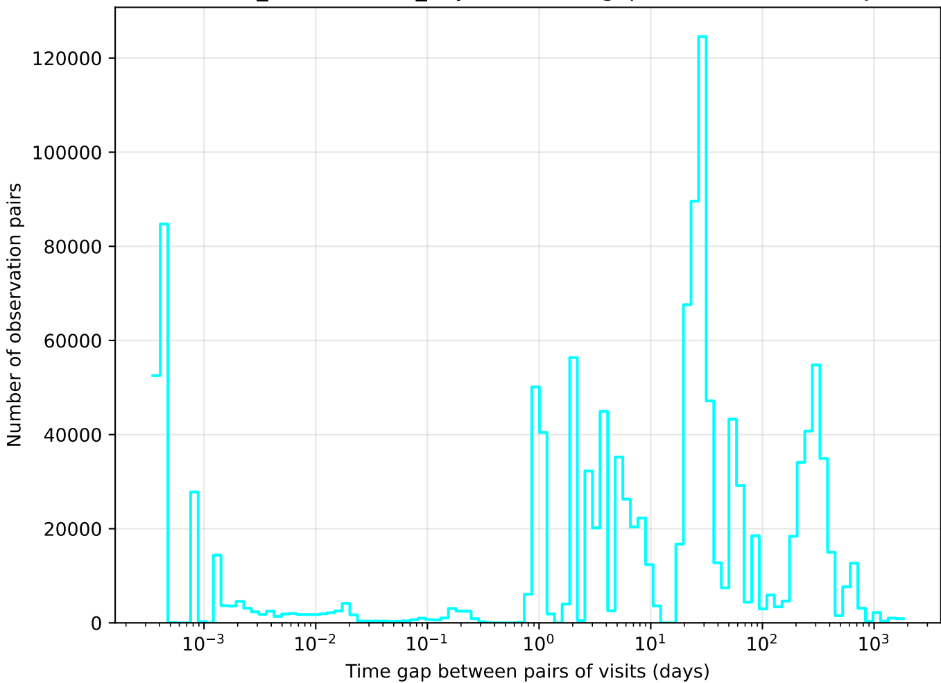
weather_cloudso0v3.4_10yrs u band: Tgaps observationStartMJD
