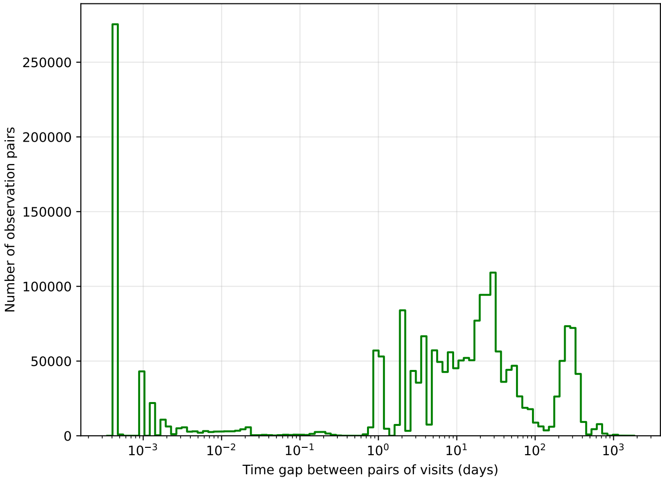
weather_cloudso0v3.4_10yrs g band: Tgaps observationStartMJD
