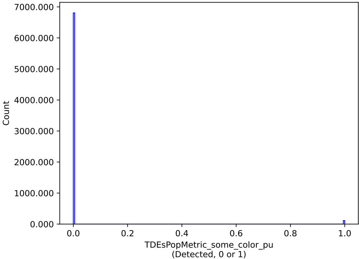
weather_cloudso0v3.4_10yrs : TDEsPopMetric_some_color_pu
