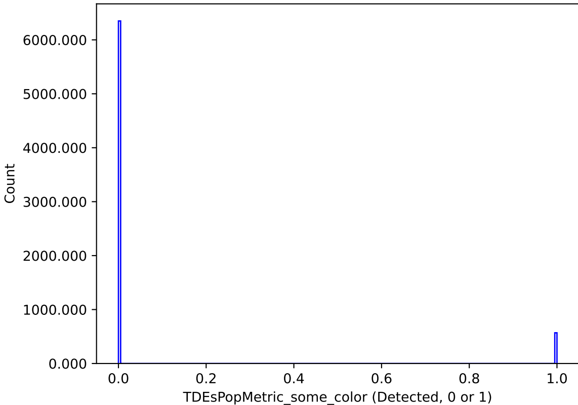
weather_cloudso0v3.4_10yrs : TDEsPopMetric_some_color
