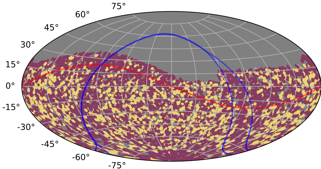
weather_cloudso0v3.4_10yrs : TDEsPopMetric_prepeak
