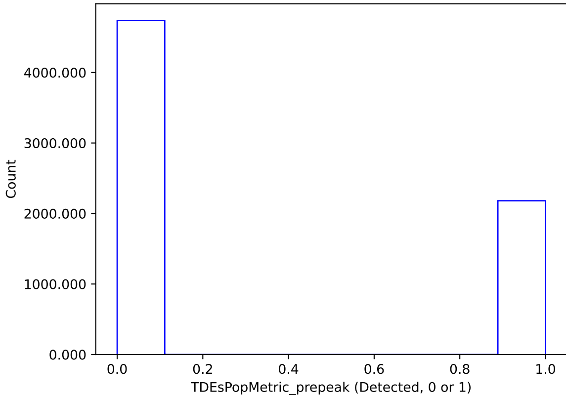
weather_cloudso0v3.4_10yrs : TDEsPopMetric_prepeak
