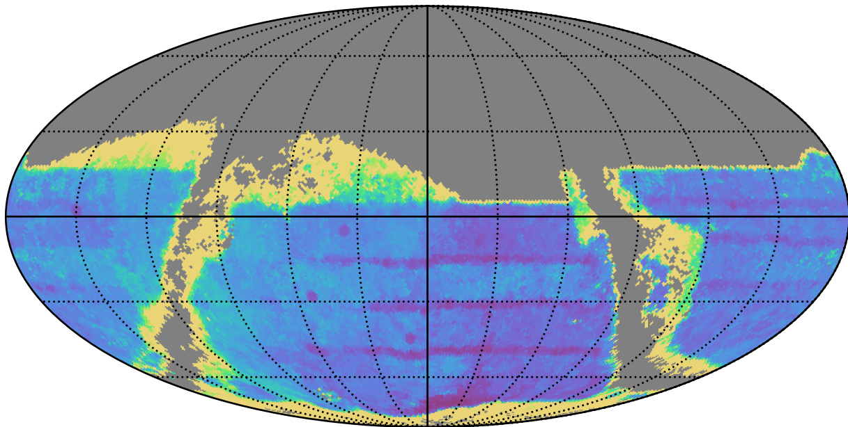
weather_cloudso0v3.4_10yrs : TDC_accuracy
