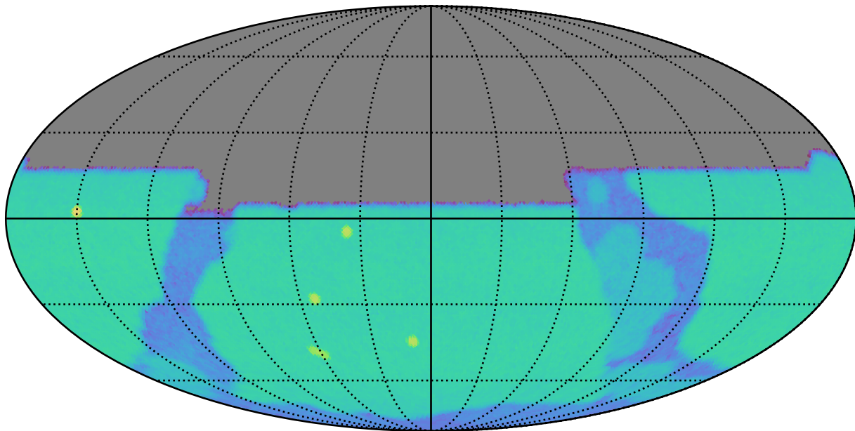
weather_cloudso0v3.4_10yrs u: SurfaceBrightLimit
