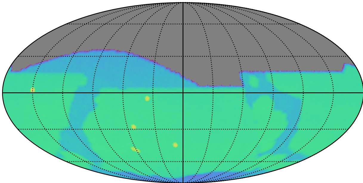
weather_cloudso0v3.4_10yrs r: SurfaceBrightLimit
