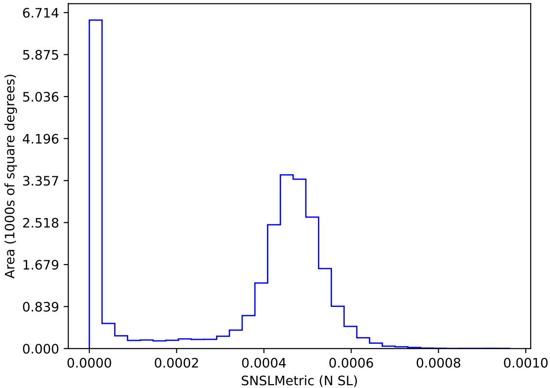
weather_cloudso0v3.4_10yrs : SNSLMetric
