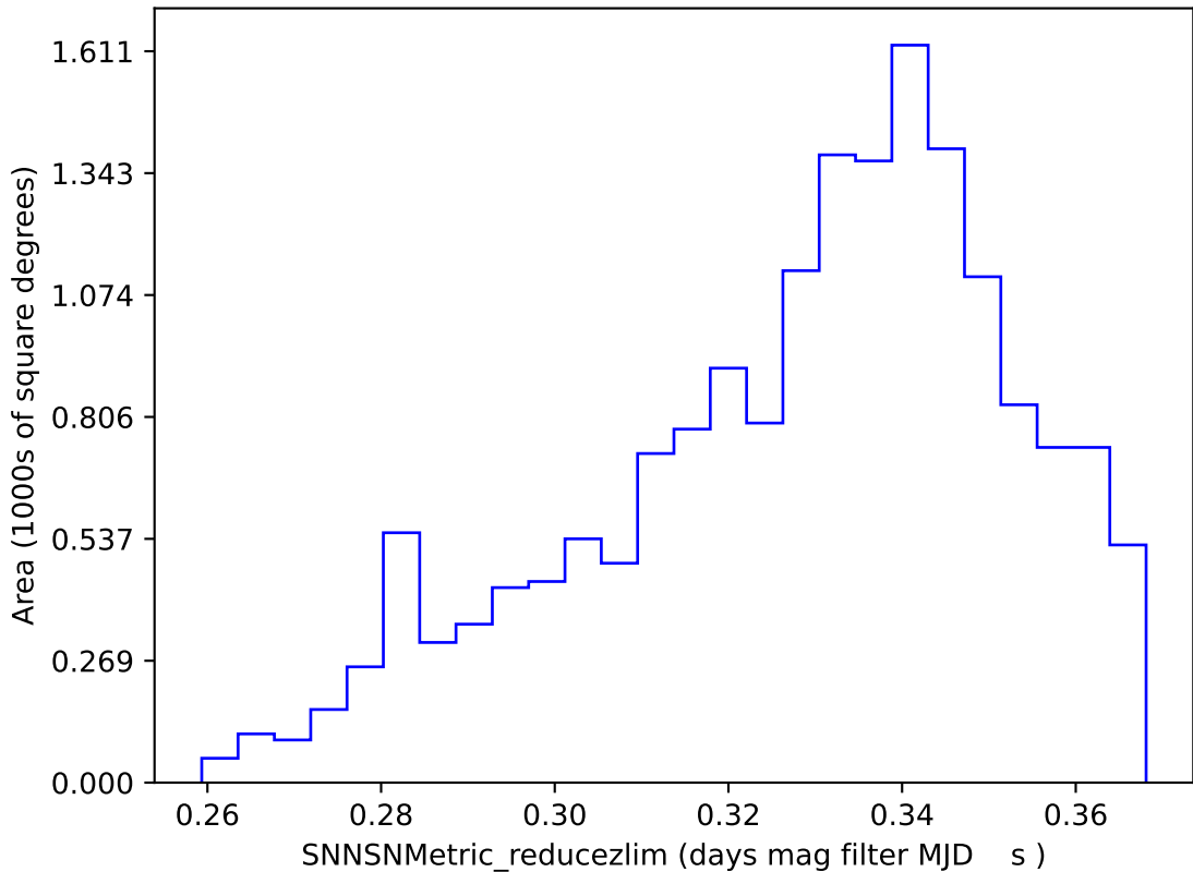
weather_cloudso0v3.4_10yrs DDF excluded: SNNSNMetric_reducezlim
