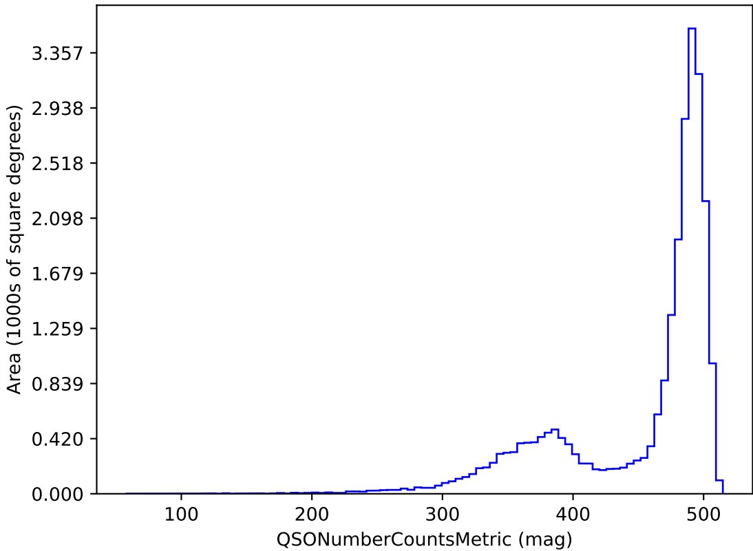
weather_cloudso0v3.4_10yrs z band and non-DD: QSONumberCountsMetric
