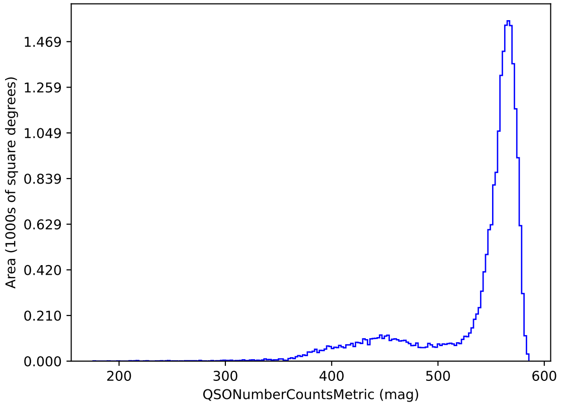
weather_cloudso0v3.4_10yrs y band and non-DD: QSONumberCountsMetric
