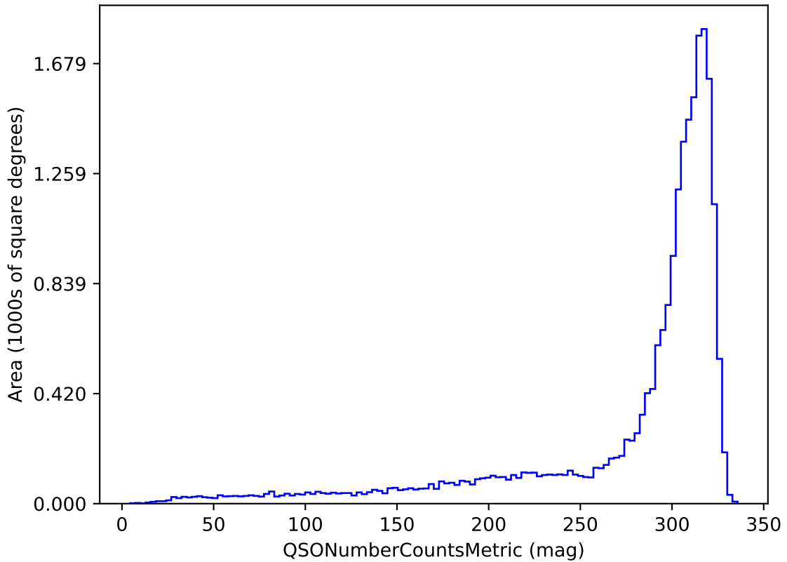
weather_cloudso0v3.4_10yrs u band and non-DD: QSONumberCountsMetric
