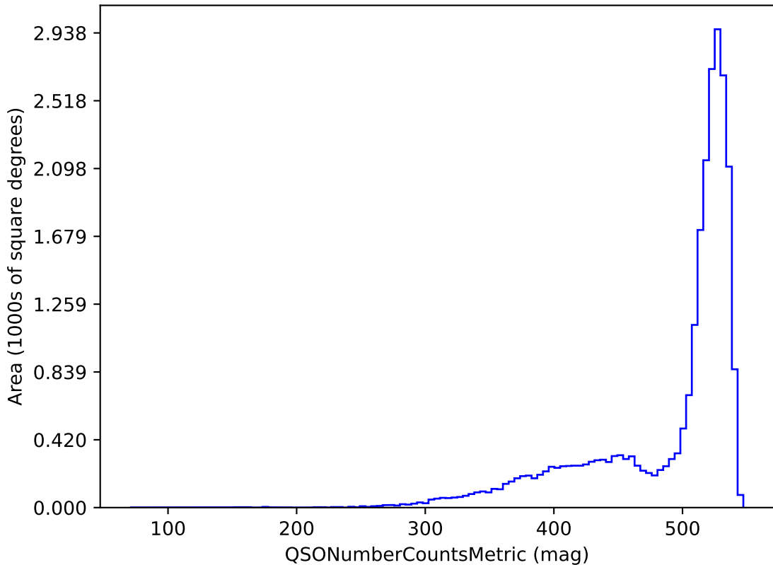
weather_cloudso0v3.4_10yrs r band and non-DD: QSONumberCountsMetric
