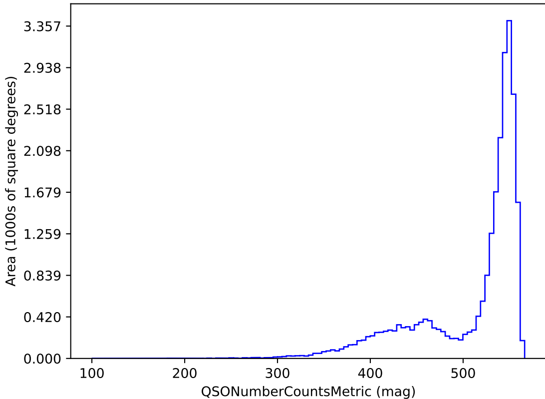
weather_cloudso0v3.4_10yrs i band and non-DD: QSONumberCountsMetric
