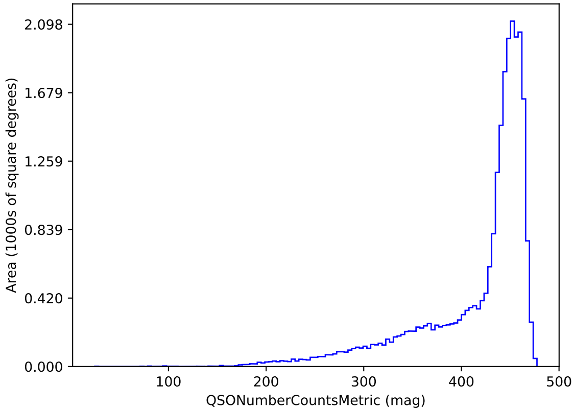
weather_cloudso0v3.4_10yrs g band and non-DD: QSONumberCountsMetric
