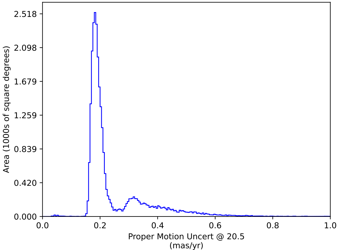
weather_cloudso0v3.4_10yrs : Proper Motion Uncert @ 20.5
