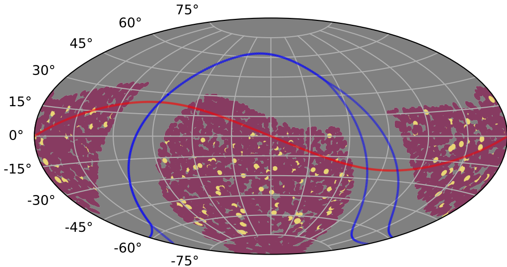
weather_cloudso0v3.4_10yrs : PrestoKNe_score_s
