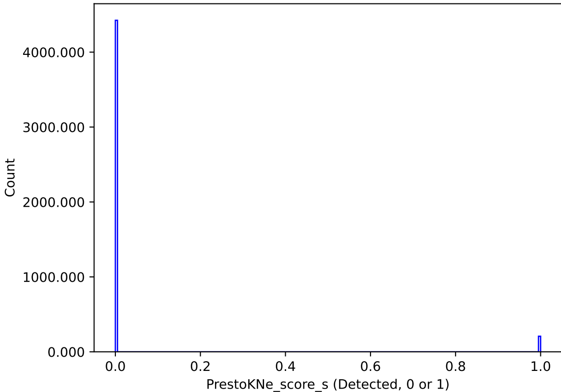
weather_cloudso0v3.4_10yrs : PrestoKNe_score_s
