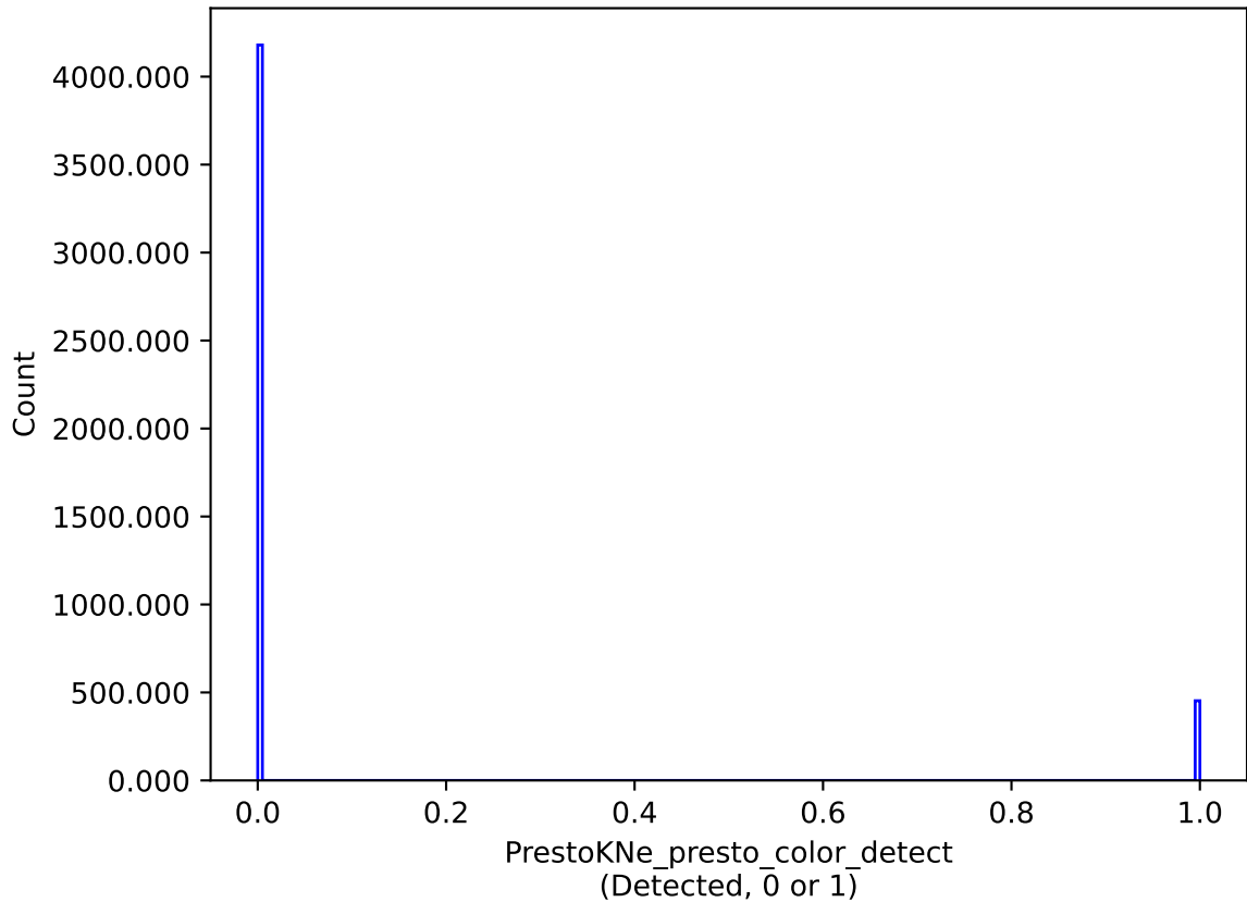
weather_cloudso0v3.4_10yrs : PrestoKNe_presto_color_detect
