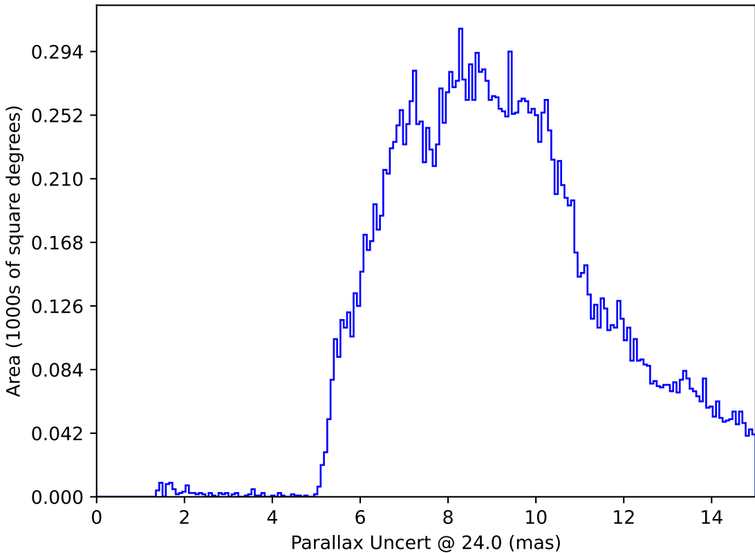
weather_cloudso0v3.4_10yrs : Parallax Uncert @ 24.0
