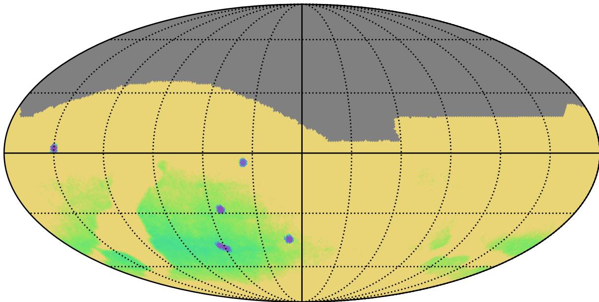
weather_cloudso0v3.4_10yrs : Parallax Uncert @ 22.4
