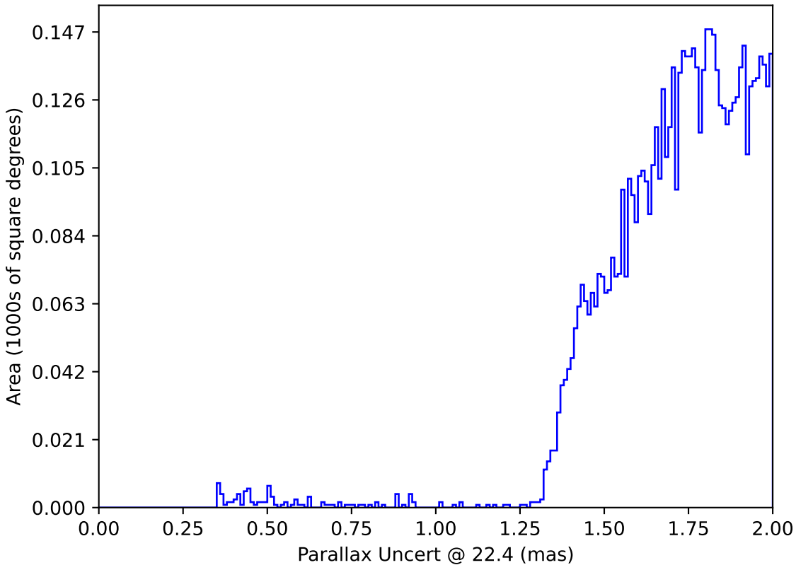
weather_cloudso0v3.4_10yrs : Parallax Uncert @ 22.4
