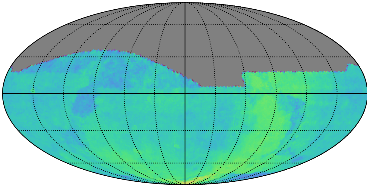
weather_cloudso0v3.4_10yrs : Parallax Coverage @ 22.4
