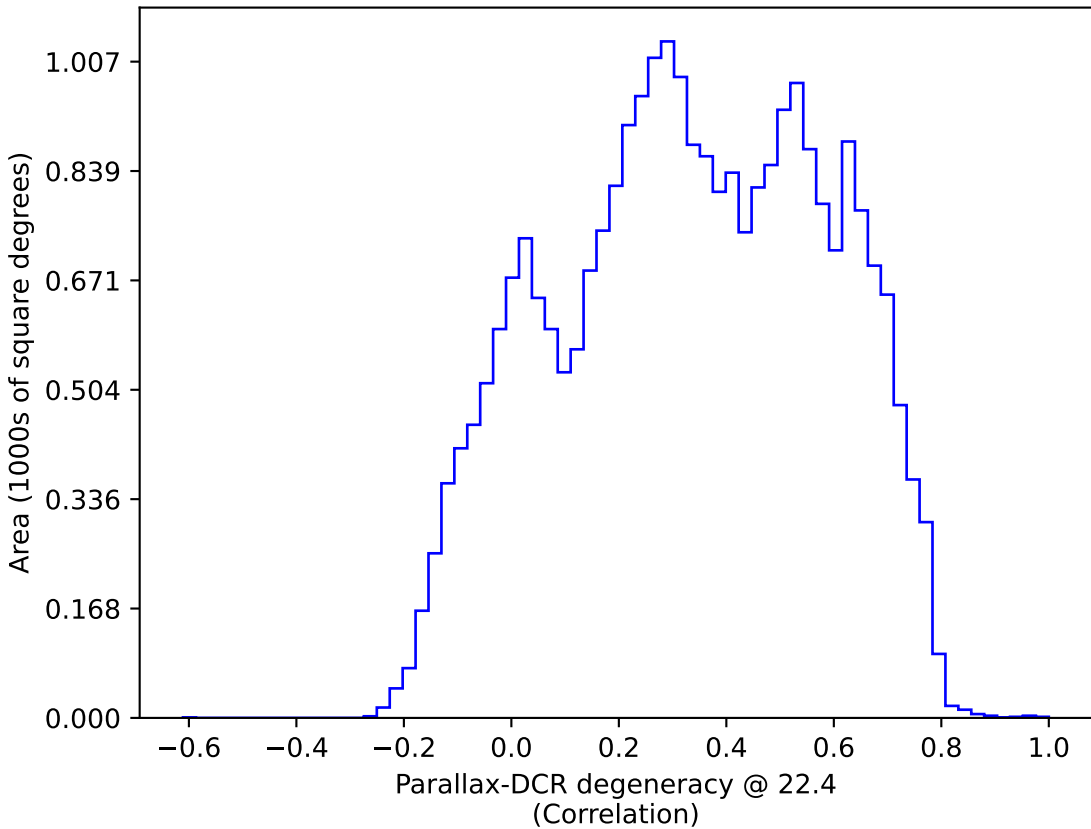
weather_cloudso0v3.4_10yrs : Parallax-DCR degeneracy @ 22.4
