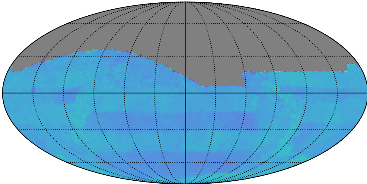
weather_cloudso0v3.4_10yrs : Normalized Proper Motion Uncert @ 24.0
