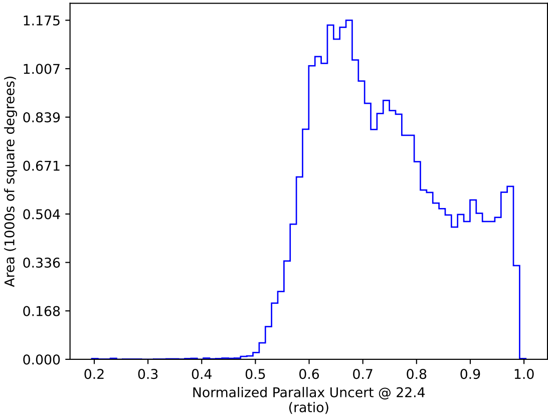
weather_cloudso0v3.4_10yrs : Normalized Parallax Uncert @ 22.4
