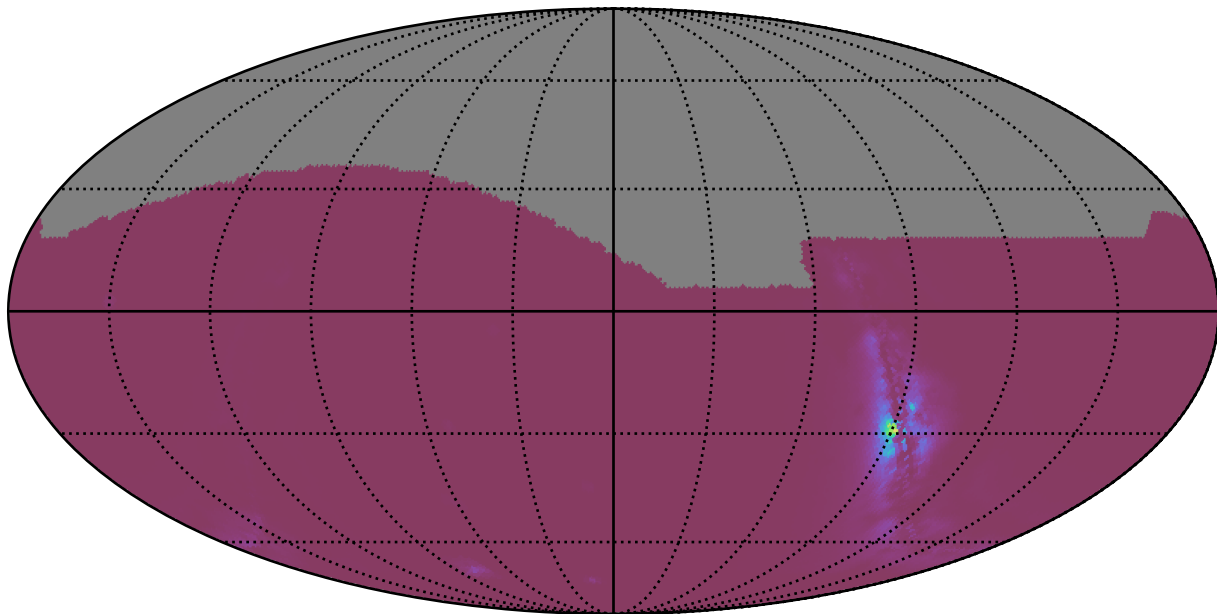
weather_cloudso0v3.4_10yrs : NlcPoints
