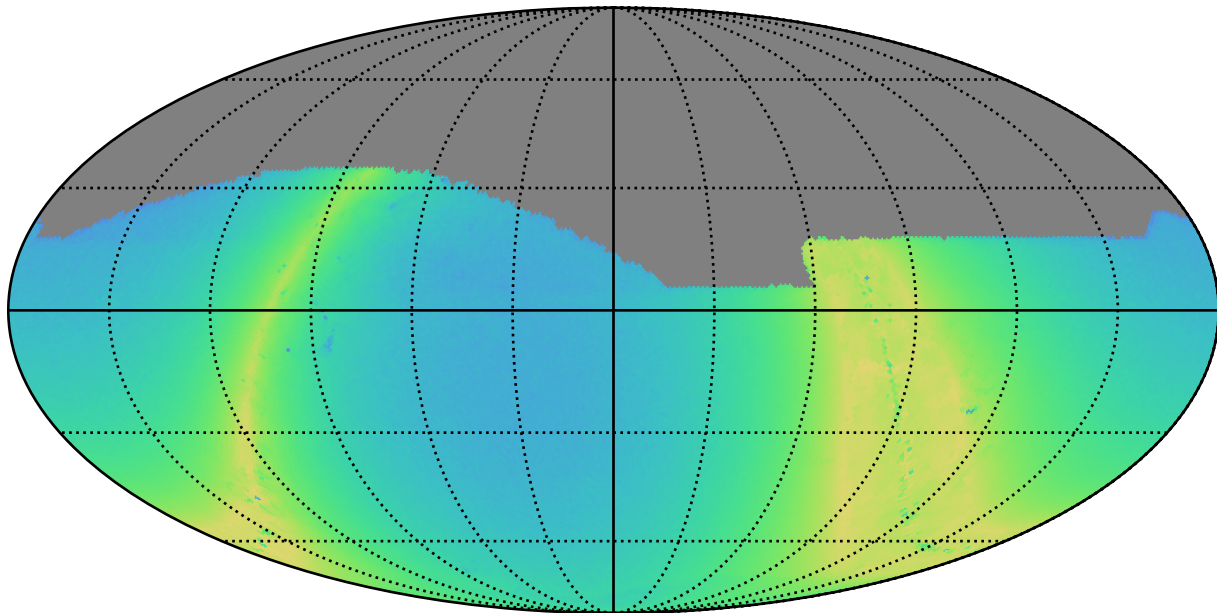
weather_cloudso0v3.4_10yrs z: N stars to Precision 0.20
