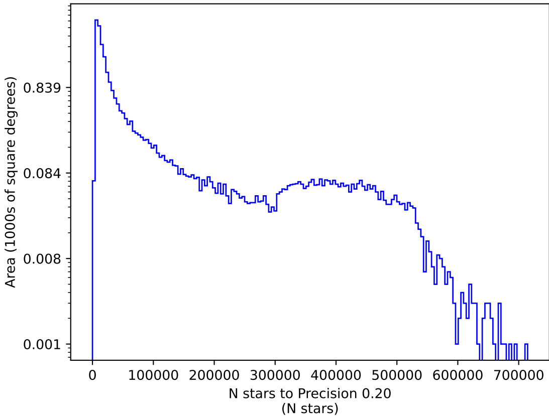
weather_cloudso0v3.4_10yrs r: N stars to Precision 0.20
