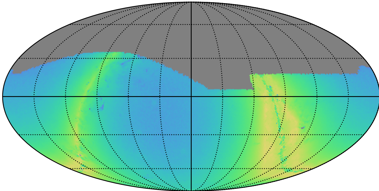
weather_cloudso0v3.4_10yrs g: N stars to Precision 0.20
