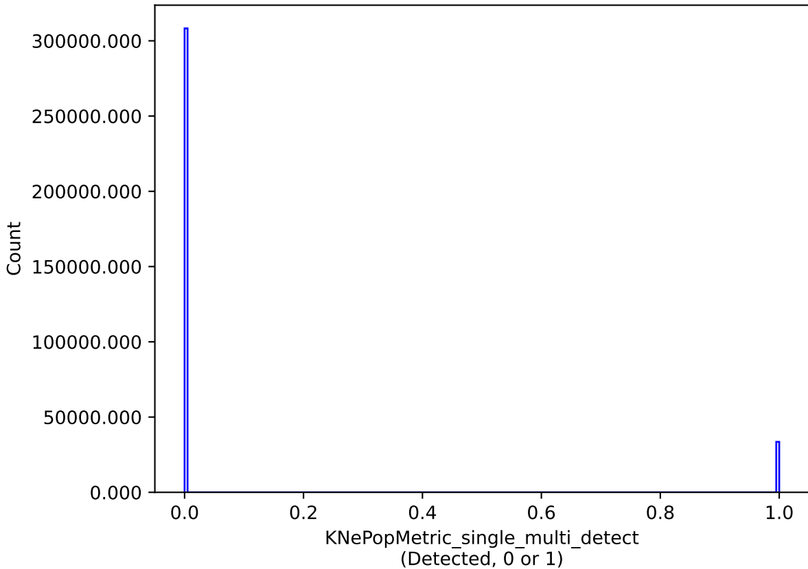
weather_cloudso0v3.4_10yrs single model: KNePopMetric_single_multi_detect
