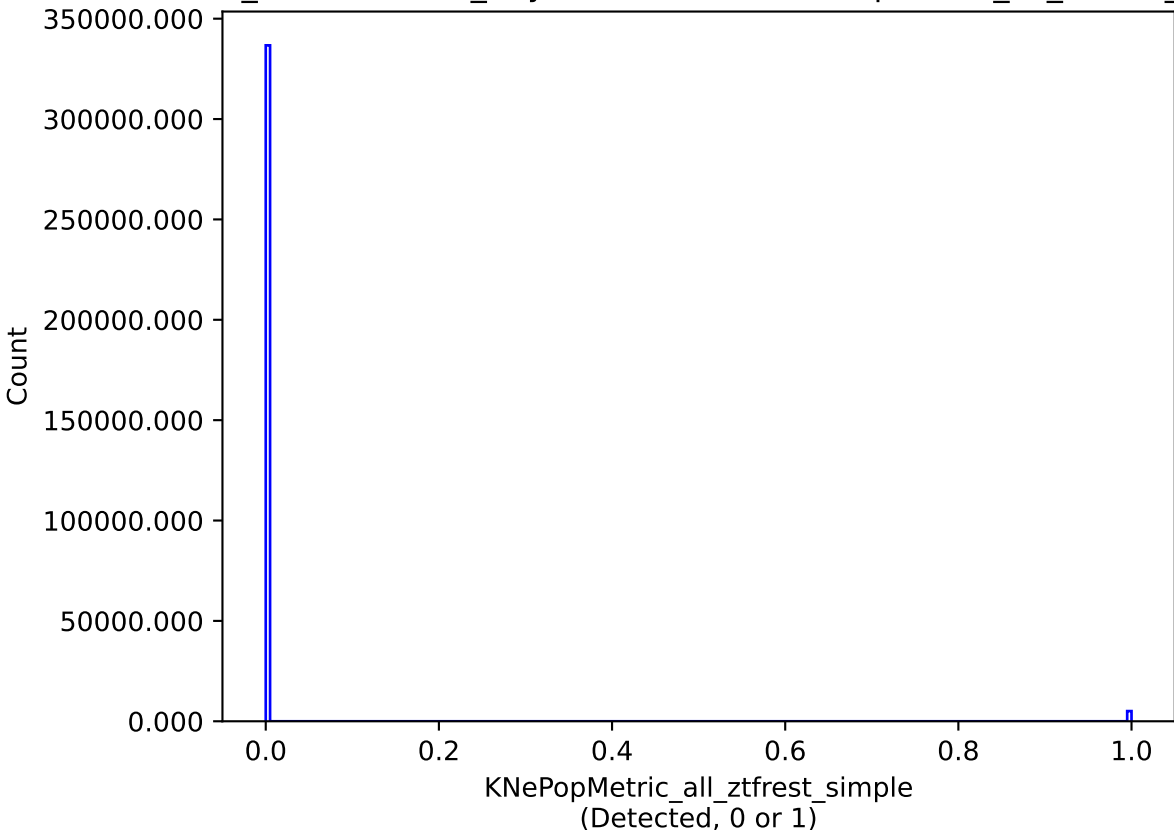
weather_cloudso0v3.4_10yrs all models: KNePopMetric_all_ztfrest_simple
