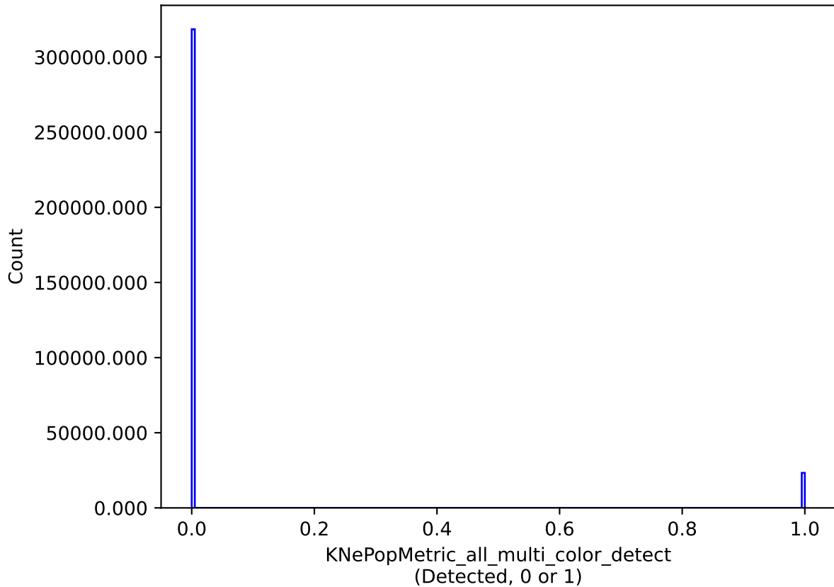
weather_cloudso0v3.4_10yrs all models: KNePopMetric_all_multi_color_detect
