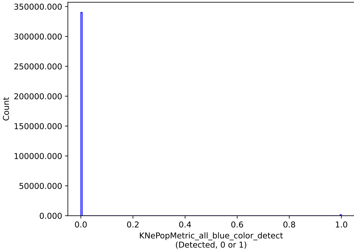
weather_cloudso0v3.4_10yrs all models: KNePopMetric_all_blue_color_detect
