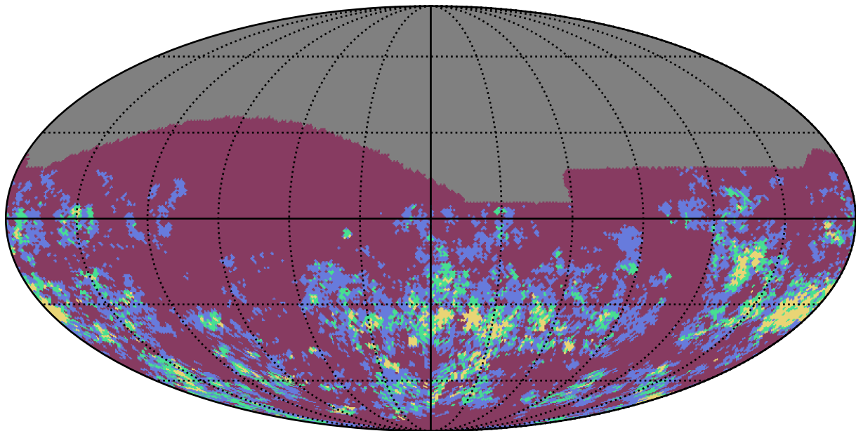
weather_cloudso0v3.4_10yrs z band: Gaps_7hr
