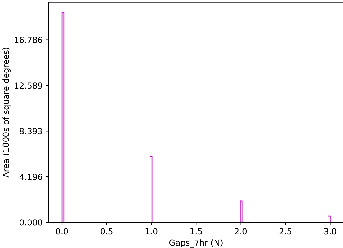
weather_cloudso0v3.4_10yrs z band: Gaps_7hr
